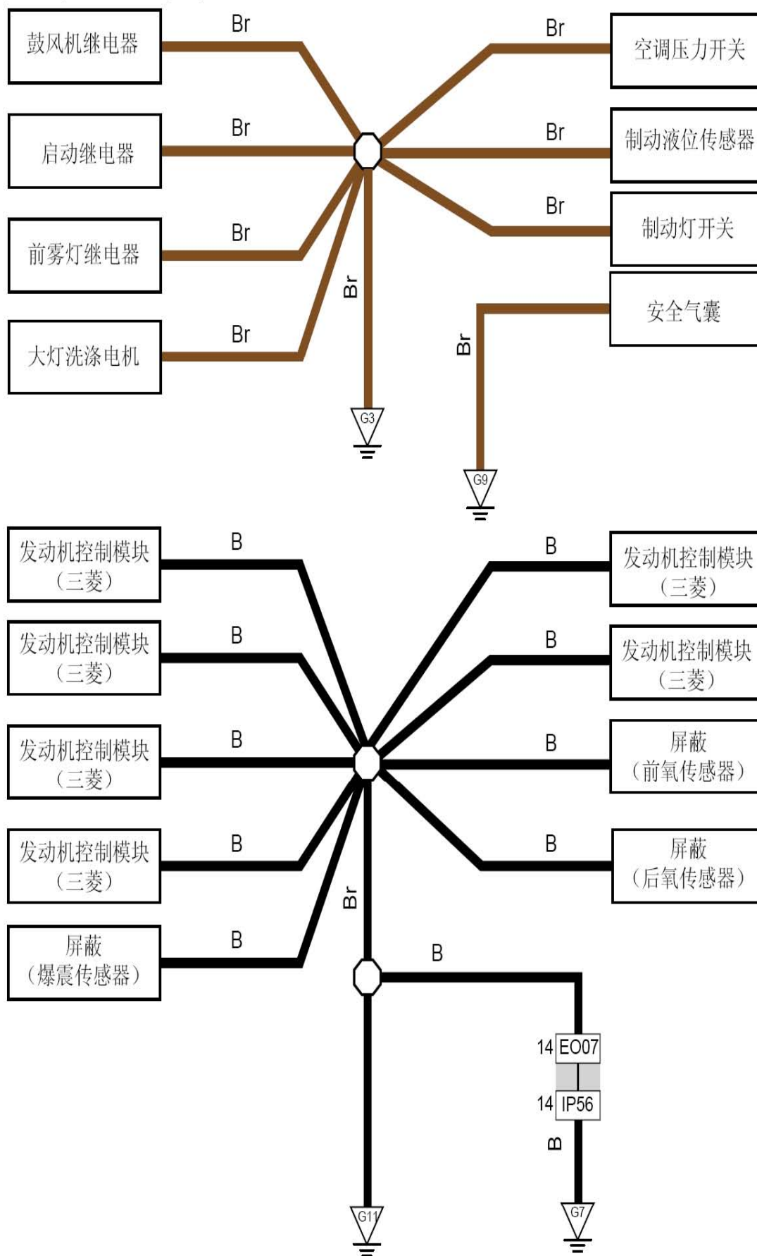
接地线路图2 (G3, G9, G7, G11)
