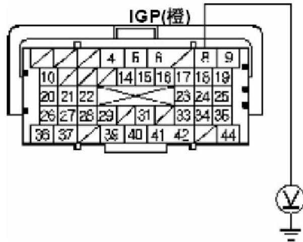
凹头插头端子侧
