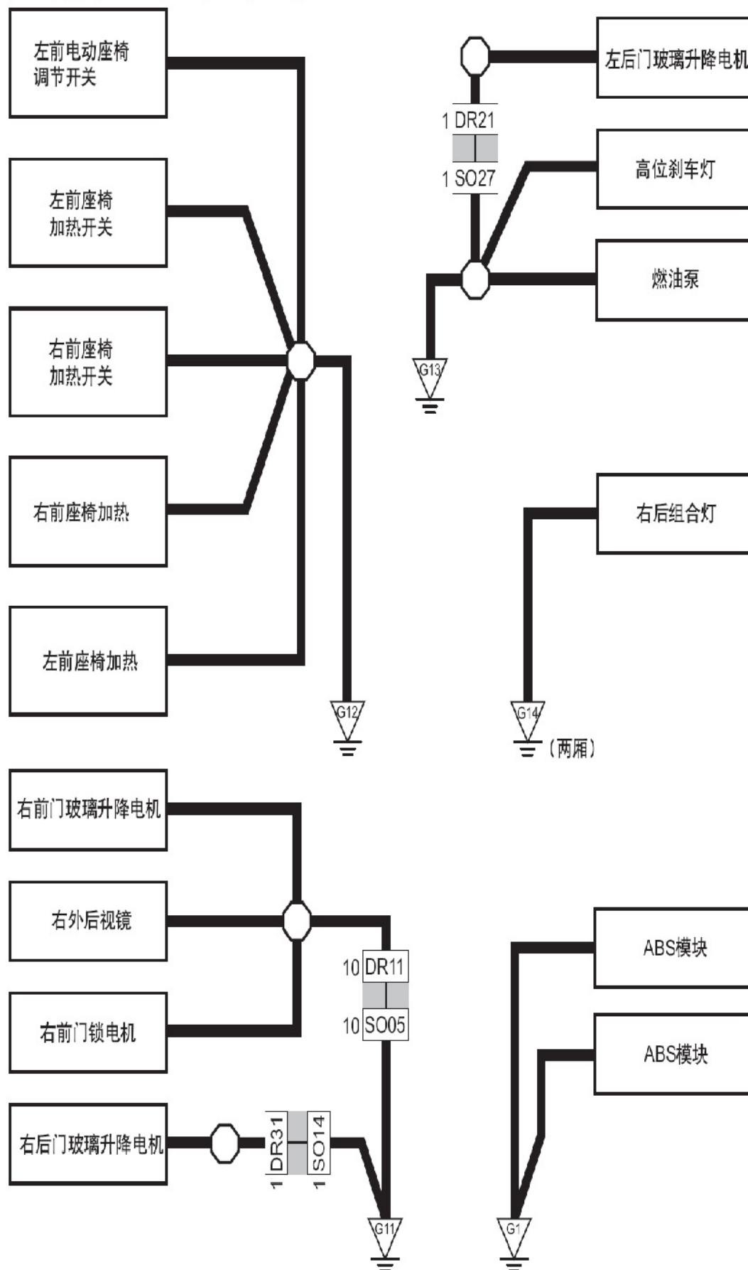
接地线路图2 (G1, G11, G12, G13, G14)
