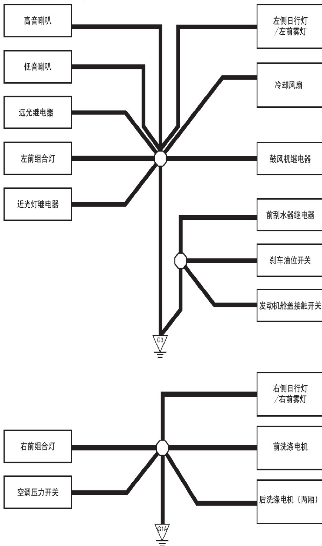
接地线路图4 (G1A, G3)
