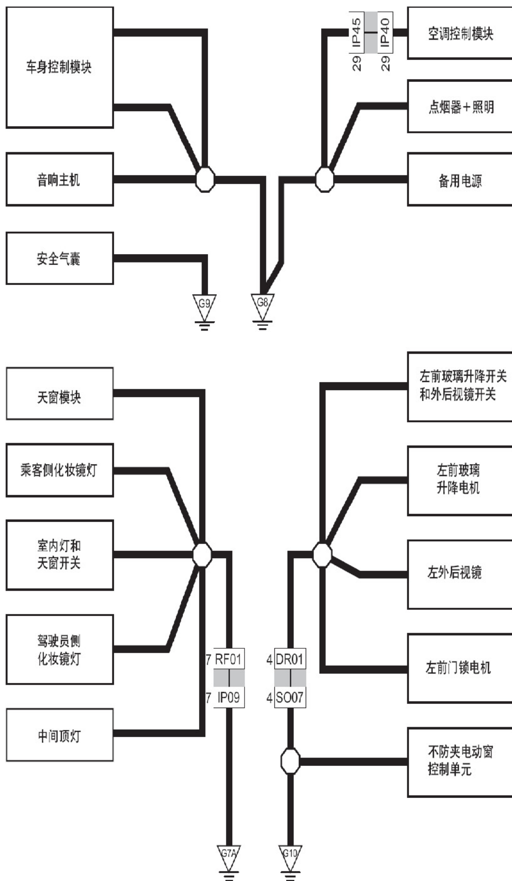
接地线路图3 (G7A, G8, G9, G10)
