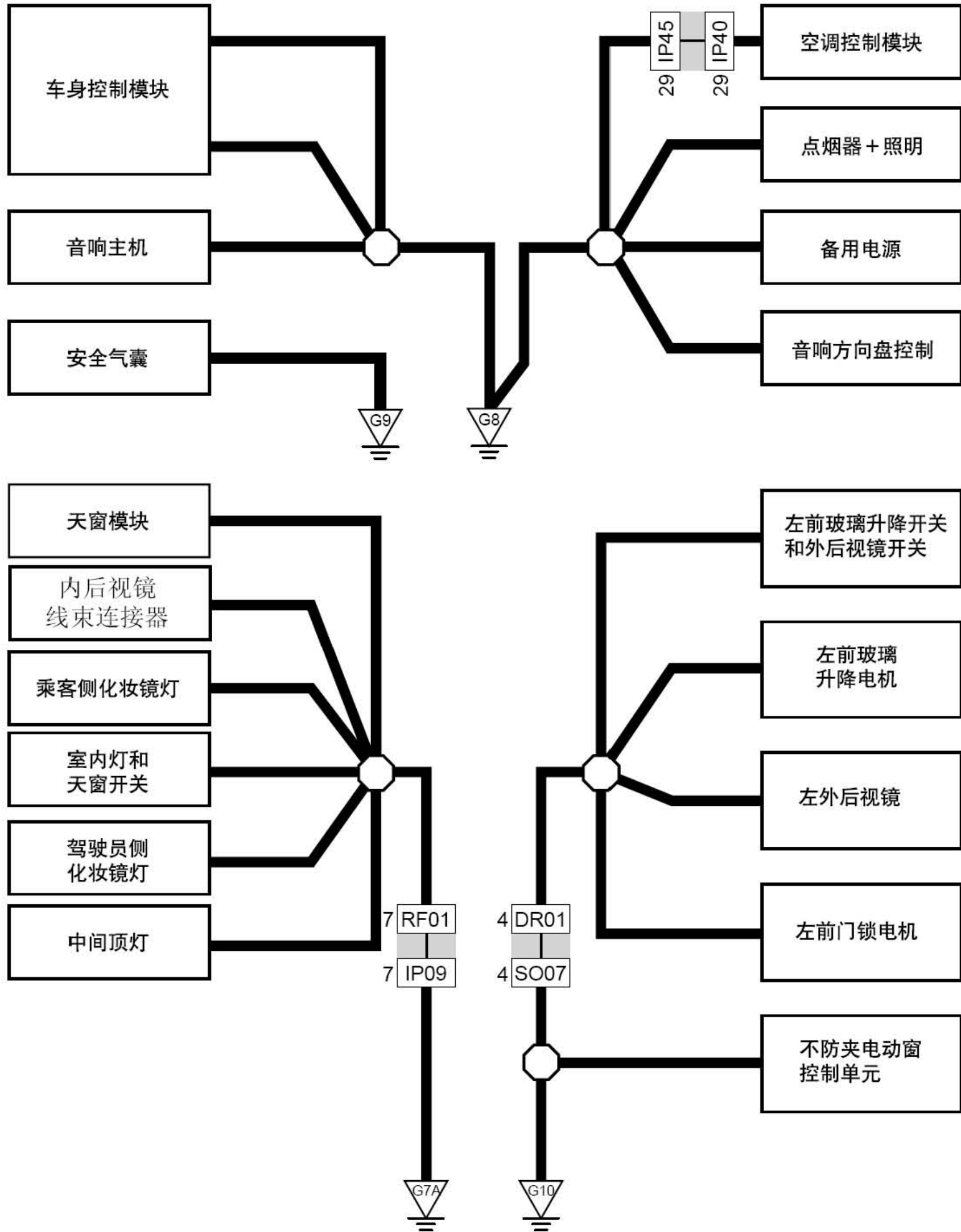
接地线路图3 (G7A, G8, G9, G10)
