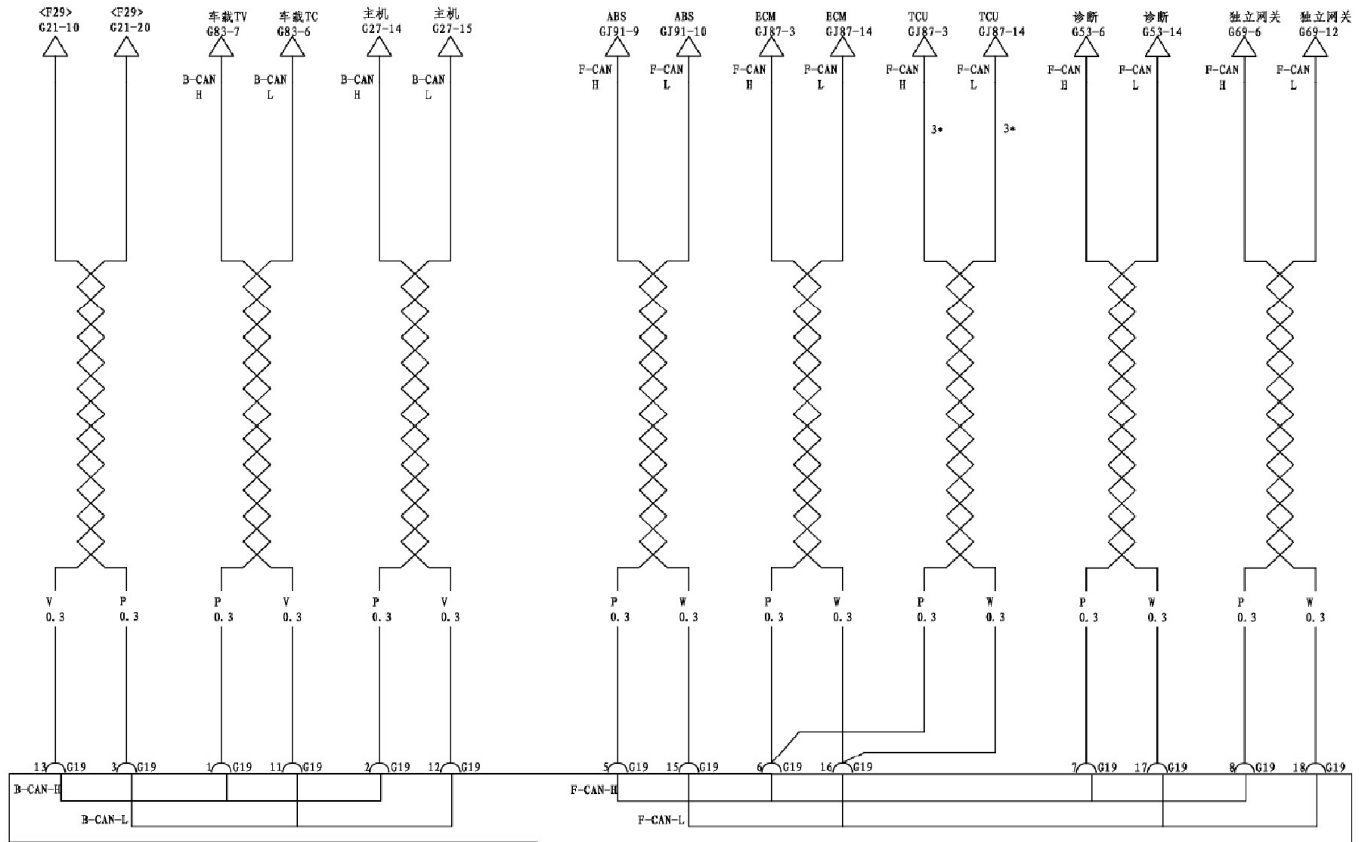
2#CAN线短接器-低速网
