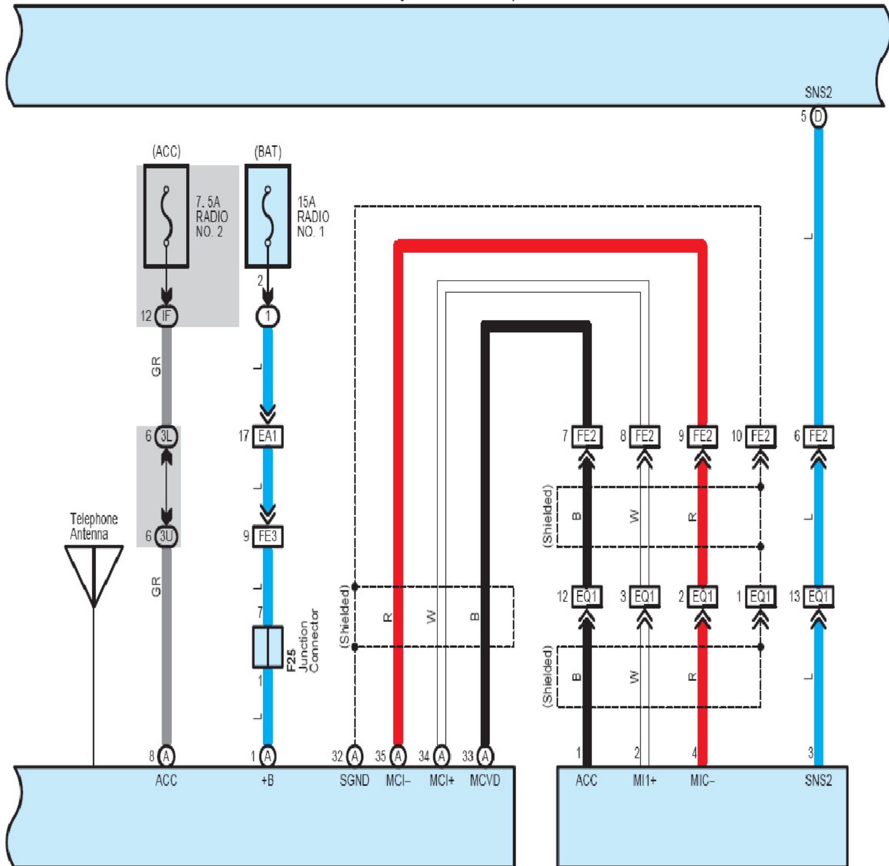
F46(A), F47(B) Telematics Transceiver
