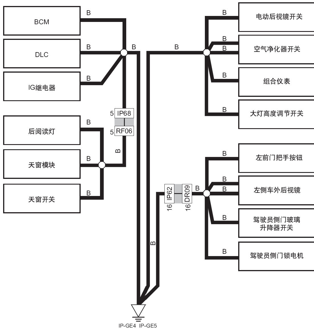
接地线路图6(IP-GE4, IP-GE5)
