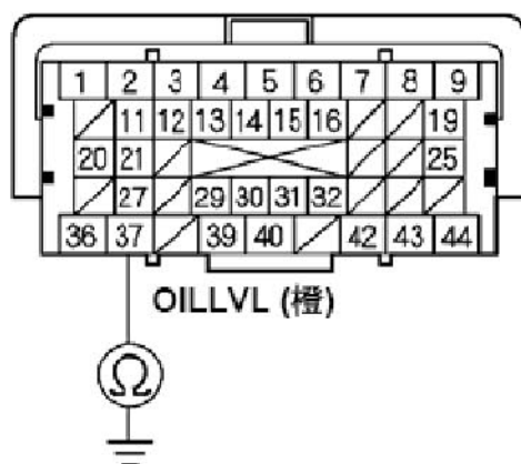
凹头插头端子侧
